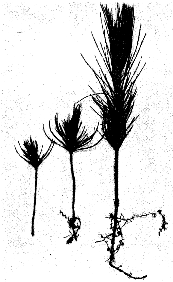
Slash pine seedlings. Left, roots destroyed entirely by the stunt nematode, Tylenchorhynchus claytoni ; center, roots partially destroyed by this nematode; right, a healthy seedling.
