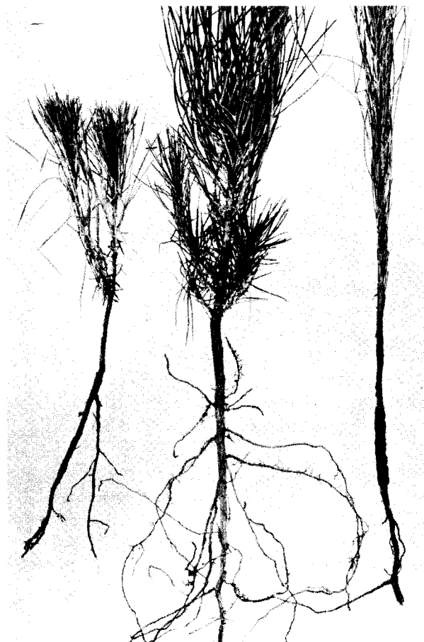
Fusiform rust swellings near ground line of 1-O loblolly pine seedlings.
