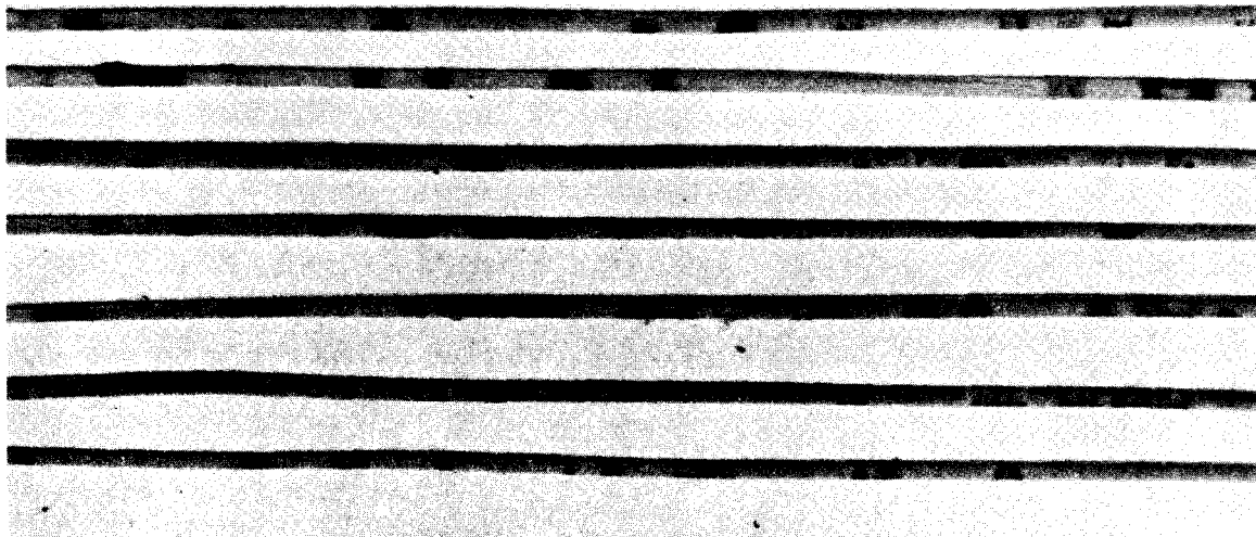
Brown spot lesions on longleaf pine needles. These are sometimes called bar-spots.
