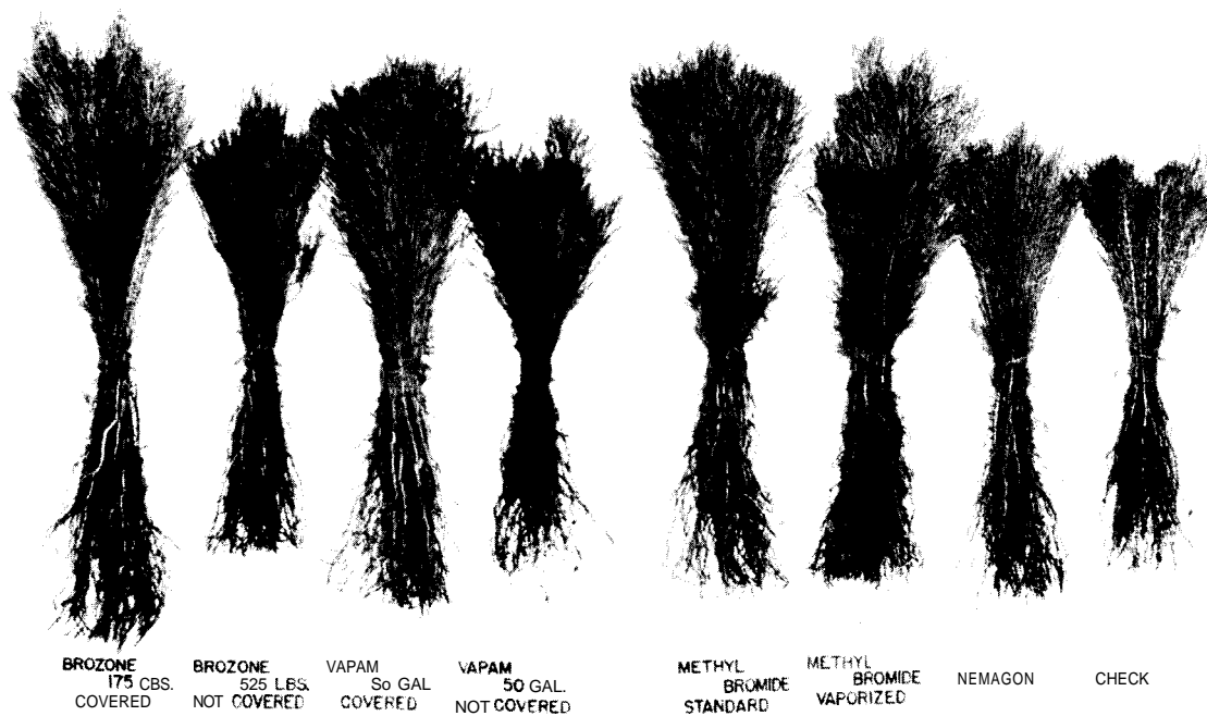
Loblolly pine seedlings from nursery beds given soil treatments as indicated. Each bundle contains 25 seedlings pulled at random from a given bed.
